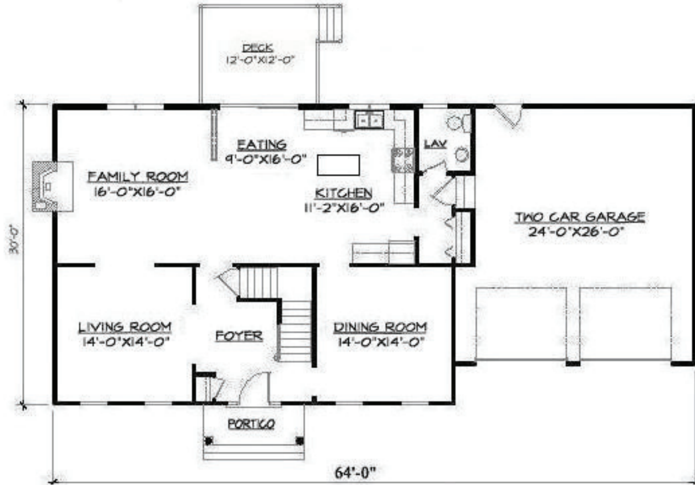
LEINOX 1ST FLOOR
