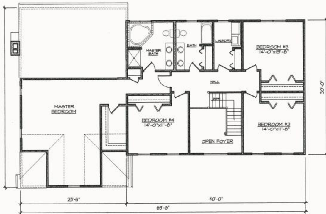
BARRINGTON 2ND FLOOR
